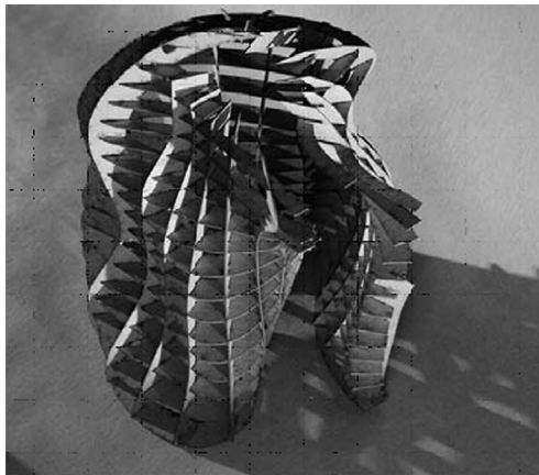
Figure 2 Output model; assembled bilateral network of ribs
